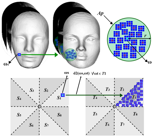
Fig. 5. Surface normal correspondence. A window of correspondence w_t is searched in the map of normals \mathbf{N}_T of the transfer object for each window w_s of the source object (face images). The region of search A_p is depicted by the circle (middle image) and is used to compute the probability distribution of the most probable window w_t that is similar to w_s . This type of correspondence works well for source and target objects that are geometrically similar. The squares at the right show the distribution of correspondence of normals based on its grouping. For each distribution w_s of sector S_i , the distribution of correspondence w_t is determined through the evaluation of a weighted distance d_2 of each distribution in T_i with w_s .
