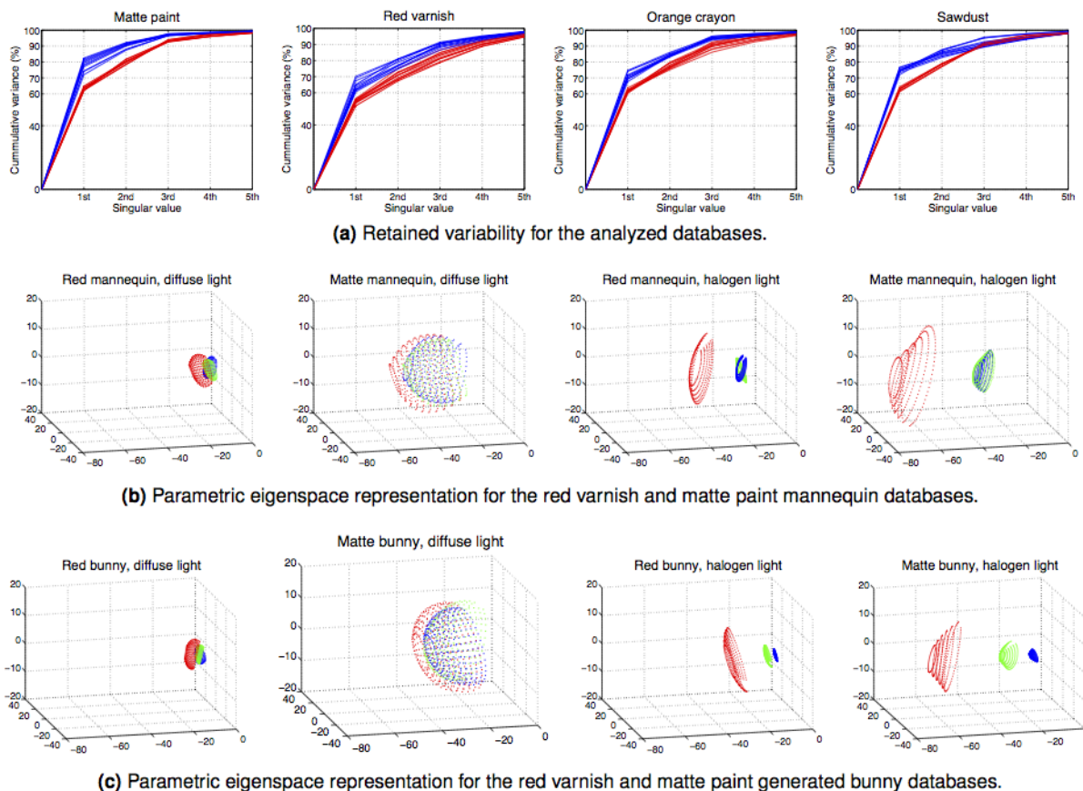
Fig. 11. Reflectance analysis in the parametric eigenspace. In (a) the retained variability of the original mannequin databases and synthetically generated databases is shown for the halogen (blue) and diffuse (red) lines. The purpose of these diagrams is to show how the databases cluster depending on the light source used in the original experiment, indicating that this information has been passed onto the target objects after transference. The results of projecting each image of the database onto the parametric eigenspace are depicted in (b) for the red varnish and matte mannequin databases (natural reflectance) and (c) for the reflectance transferred bunny databases. Each image is shown in colored dots, where the color refers to database decomposition for the red, green, and blue color channels
