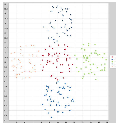
Fig. 4. Dataset spherical_5_2
